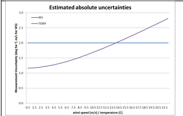
Figure 4: Absolute uncertainties for hourly wind speed and temperature.
