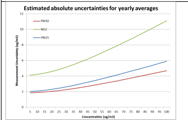
Figure 6: Absolute uncertainties for yearly PM10, PM2.5 and NO2 as a function of the concentration level.
