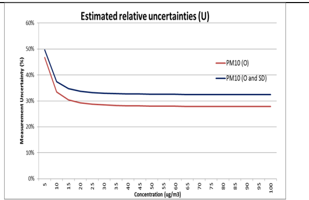
Figure 7: Comparison of daily averaged PM10 uncertainty for a single value and for an entire time series. [comparison of formulations (14) referred to as (O) in figure) and (15) referred to as (O and SD) in figure]
