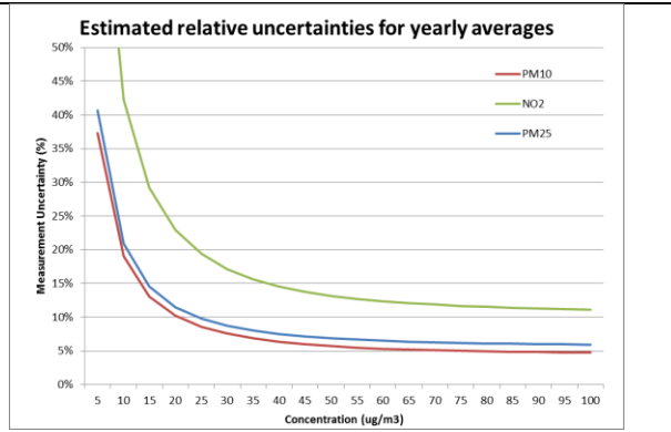
Figure 5: Relative uncertainties for yearly PM10, PM2.5 and NO2 as a function of the concentration.
